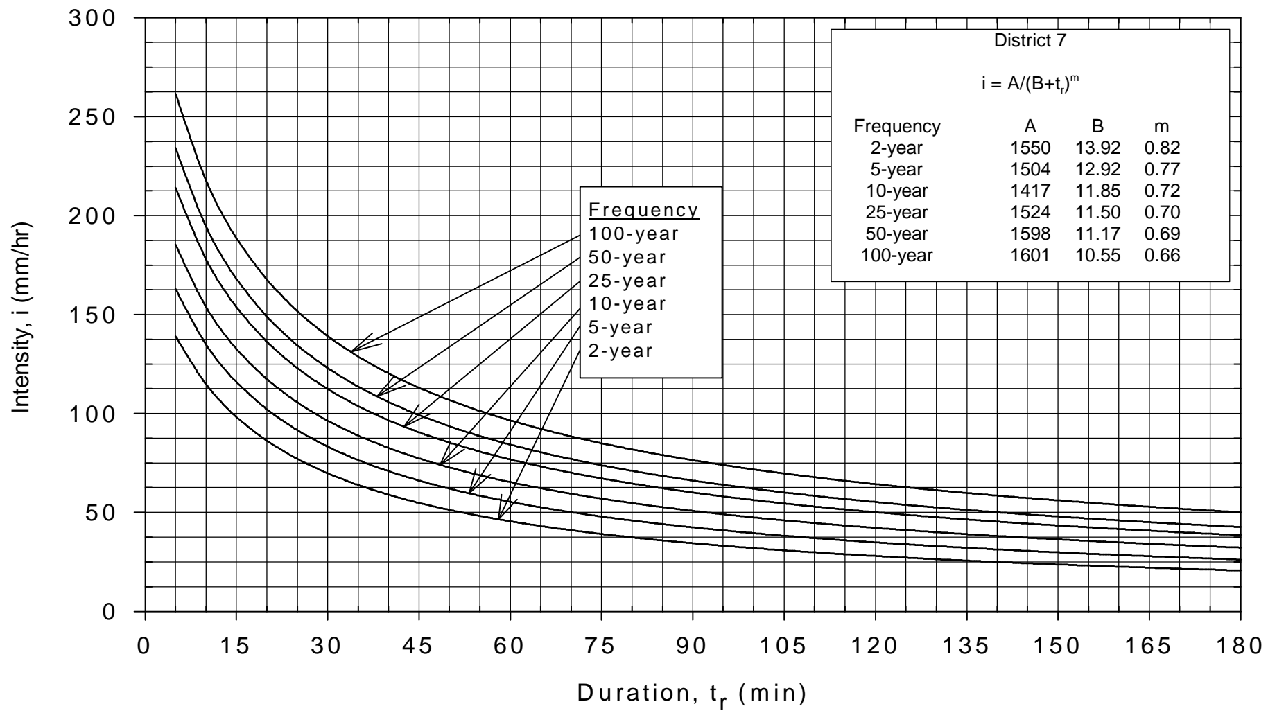
Rainfall Intensity-Duration-Frequency Curves for MoDOT District 7
