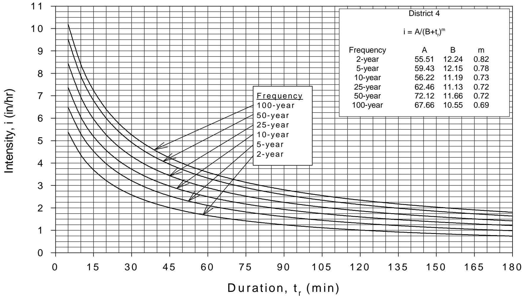
Rainfall Intensity-Duration-Frequency Curves for MoDOT District 4
