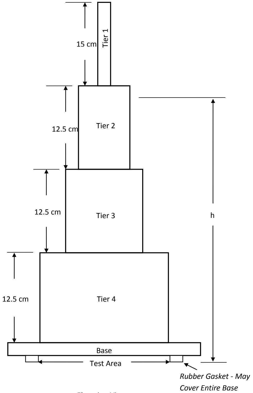
Elevation View
