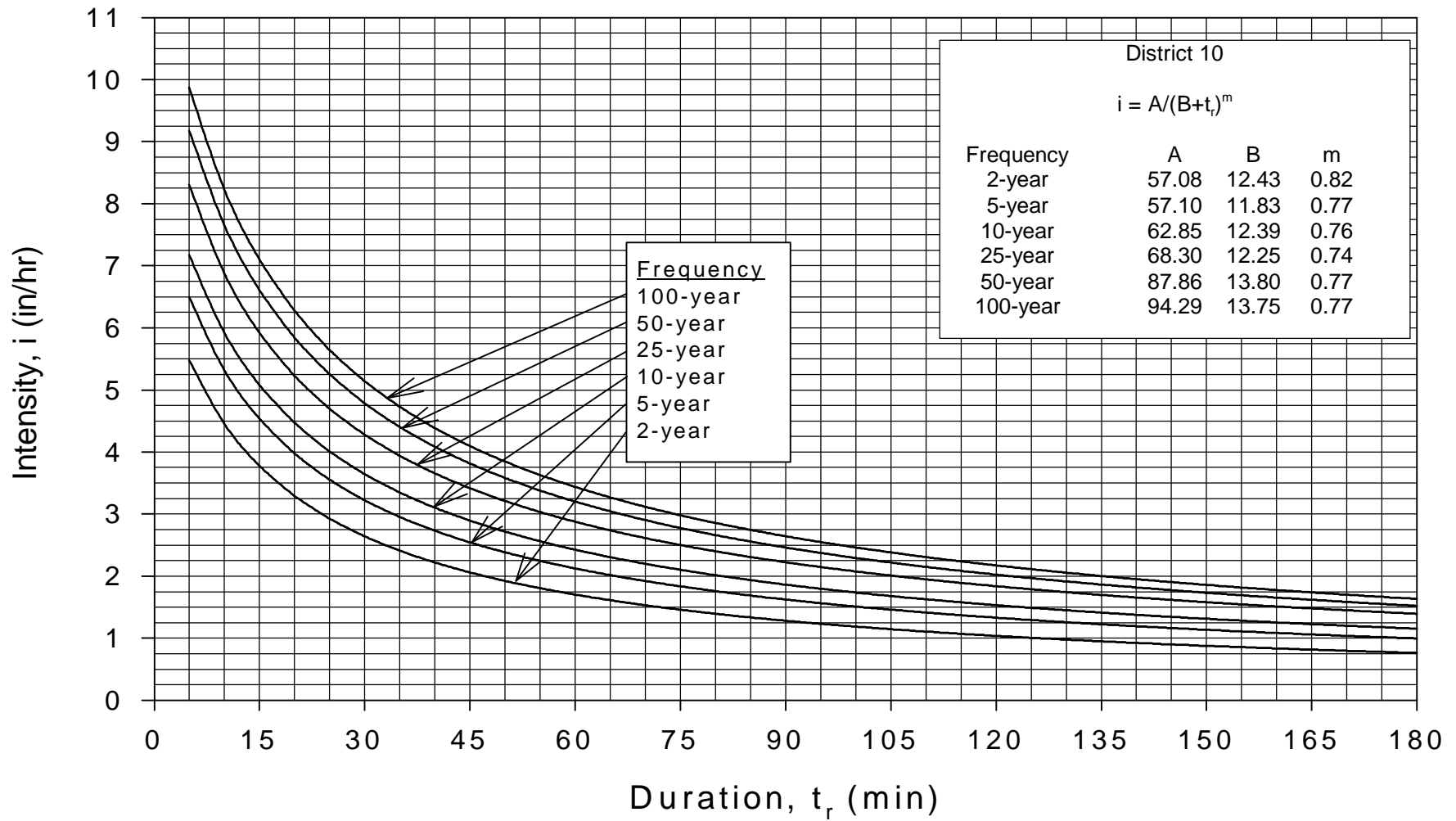
Rainfall Intensity-Duration-Frequency Curves for MoDOT District 10
