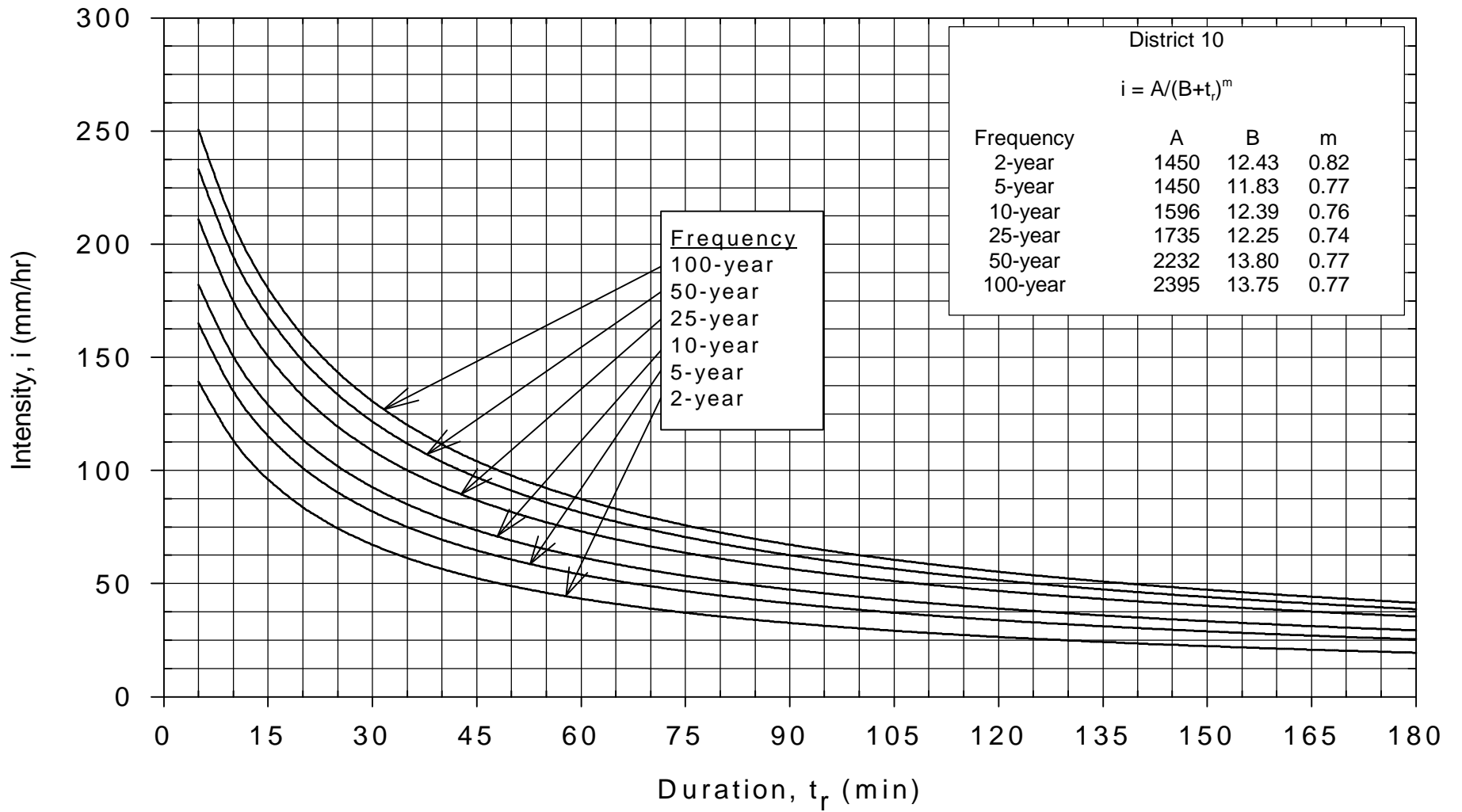
Rainfall Intensity-Duration-Frequency Curves for MoDOT District 10
