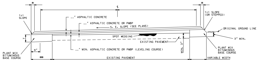
SECTION ON SUPERELEVATED CURVE
