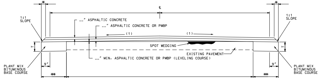
SECTION ON TANGENT
