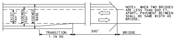
WIDTH TRANSITION AT BRIDGE TO BE RESURFACED
