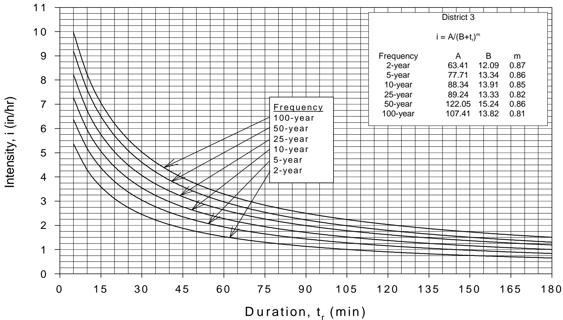
Rainfall Intensity-Duration-Frequency Curves for MoDOT District 3
