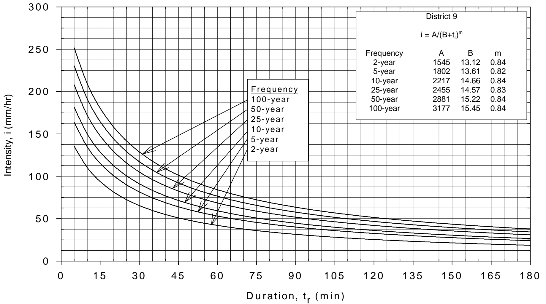
Rainfall Intensity-Duration-Frequency Curves for MoDOT District 9
