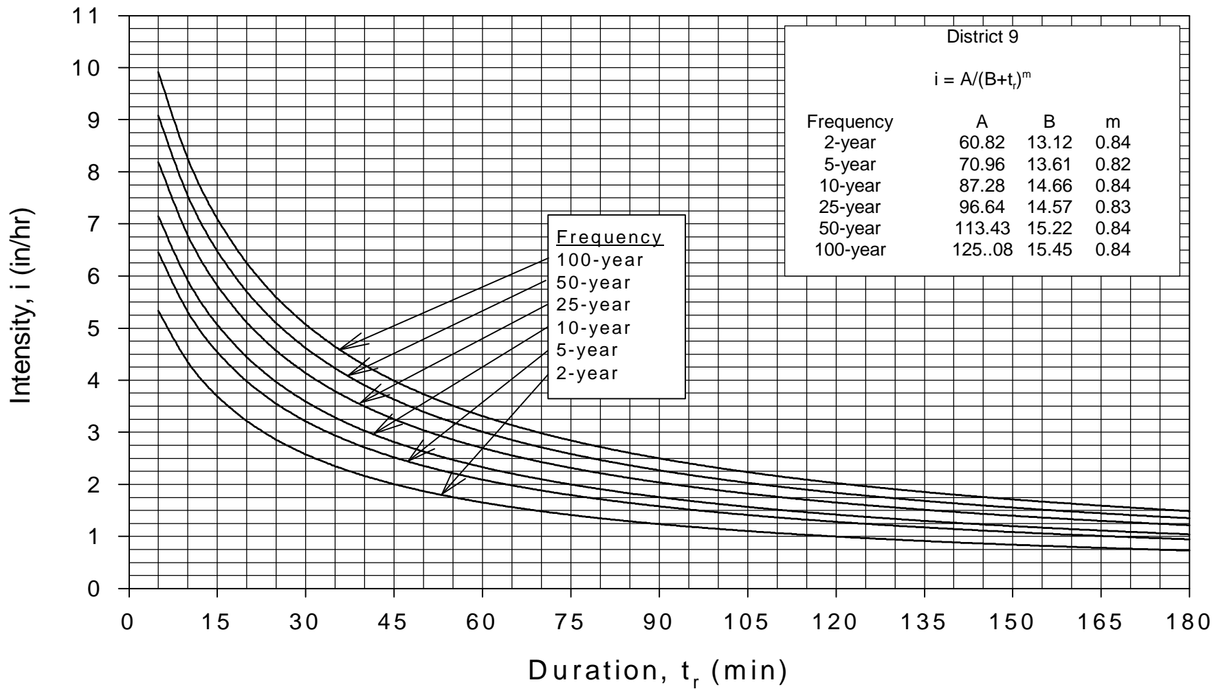
Rainfall Intensity-Duration-Frequency Curves for MoDOT District 9
