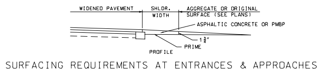
SURFACING REQUIREMENTS AT ENTRANCES & APPROACHES
