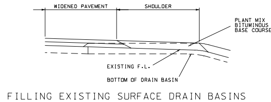
FILLING EXISTING SURFACE DRAIN BASINS
