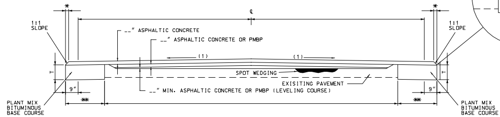
SECTION ON TANGENT (1) MATCH EXISTING
