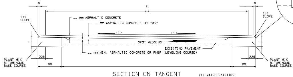
SECTION ON TANGENT
