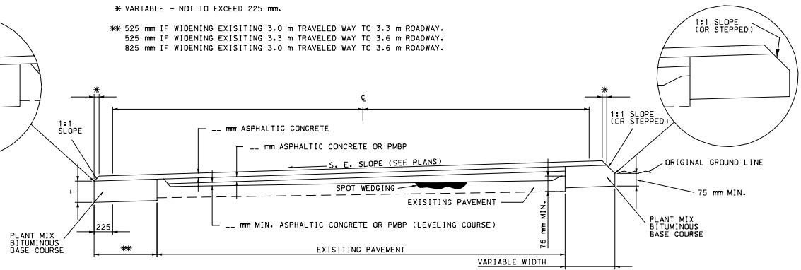
SECTION ON SUPERELEVATED CURVE
