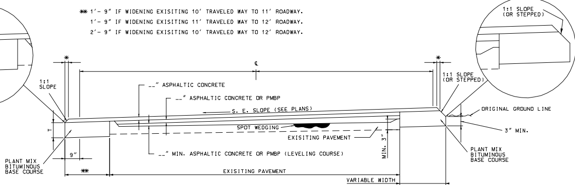
SECTION ON SUPERELEVATED CURVE
