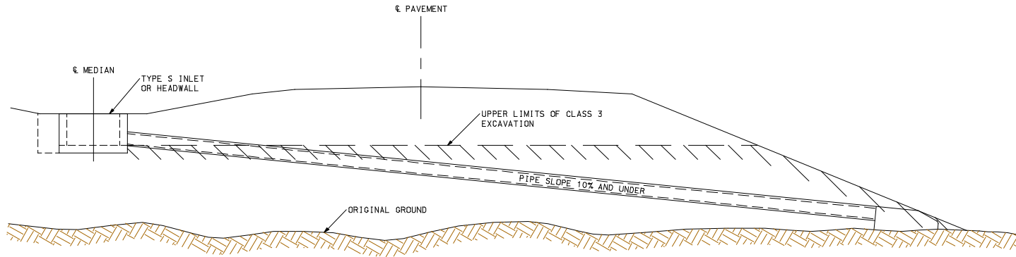
MEDIAN PIPE ON STRAIGHT ALIGNMENT USE WHEN PIPE SLOPE IS 10% OR LESS
