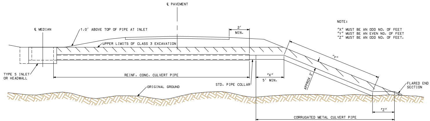
COMBINATION OF RIGID AND FLEXIBLE PIPE ON BROKEN-BACK ALIGNMENT USE WHEN PIPE SLOPE IS MORE THAN 10%
