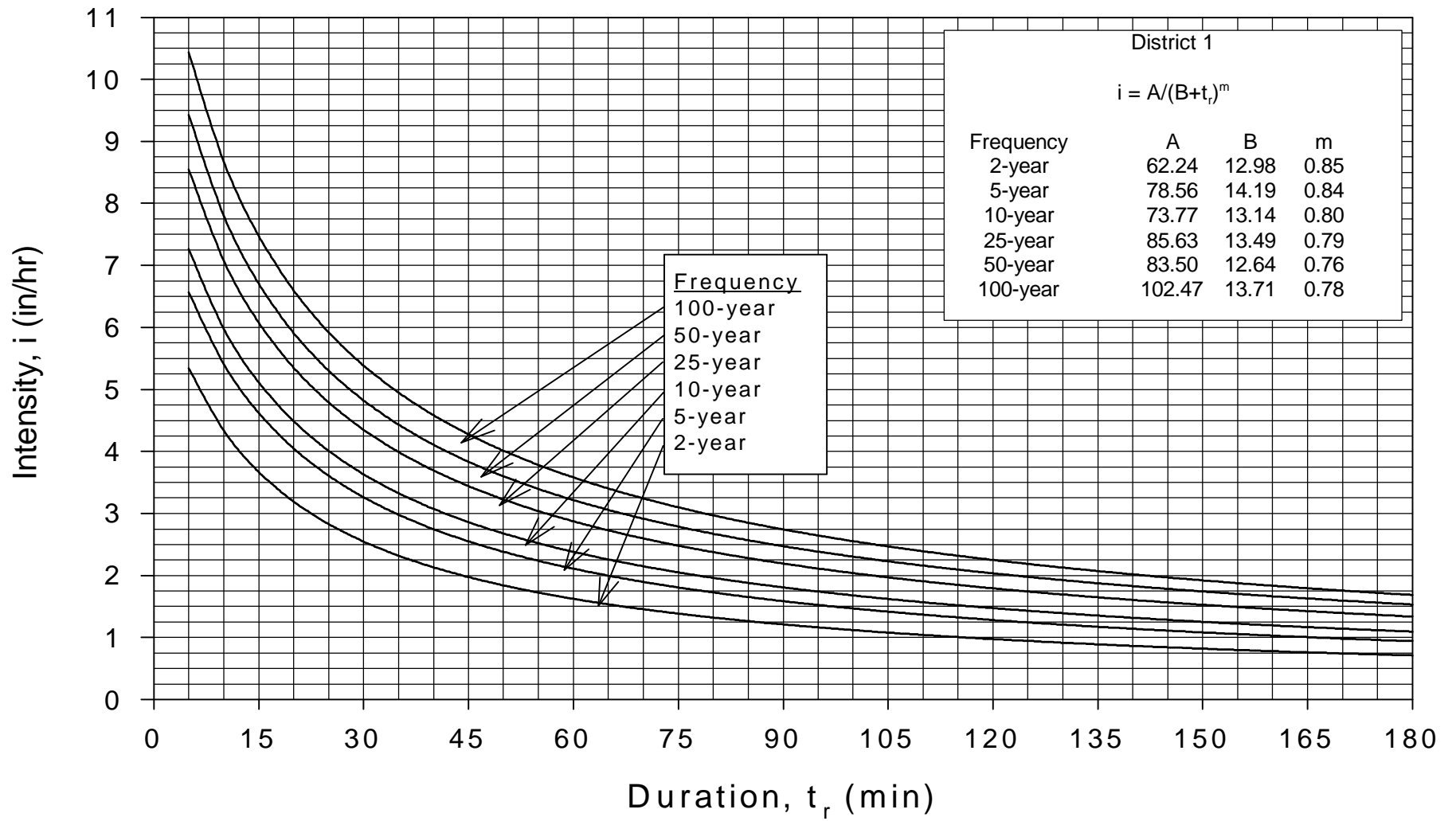
Rainfall Intensity-Duration-Frequency Curves for MoDOT District 1
