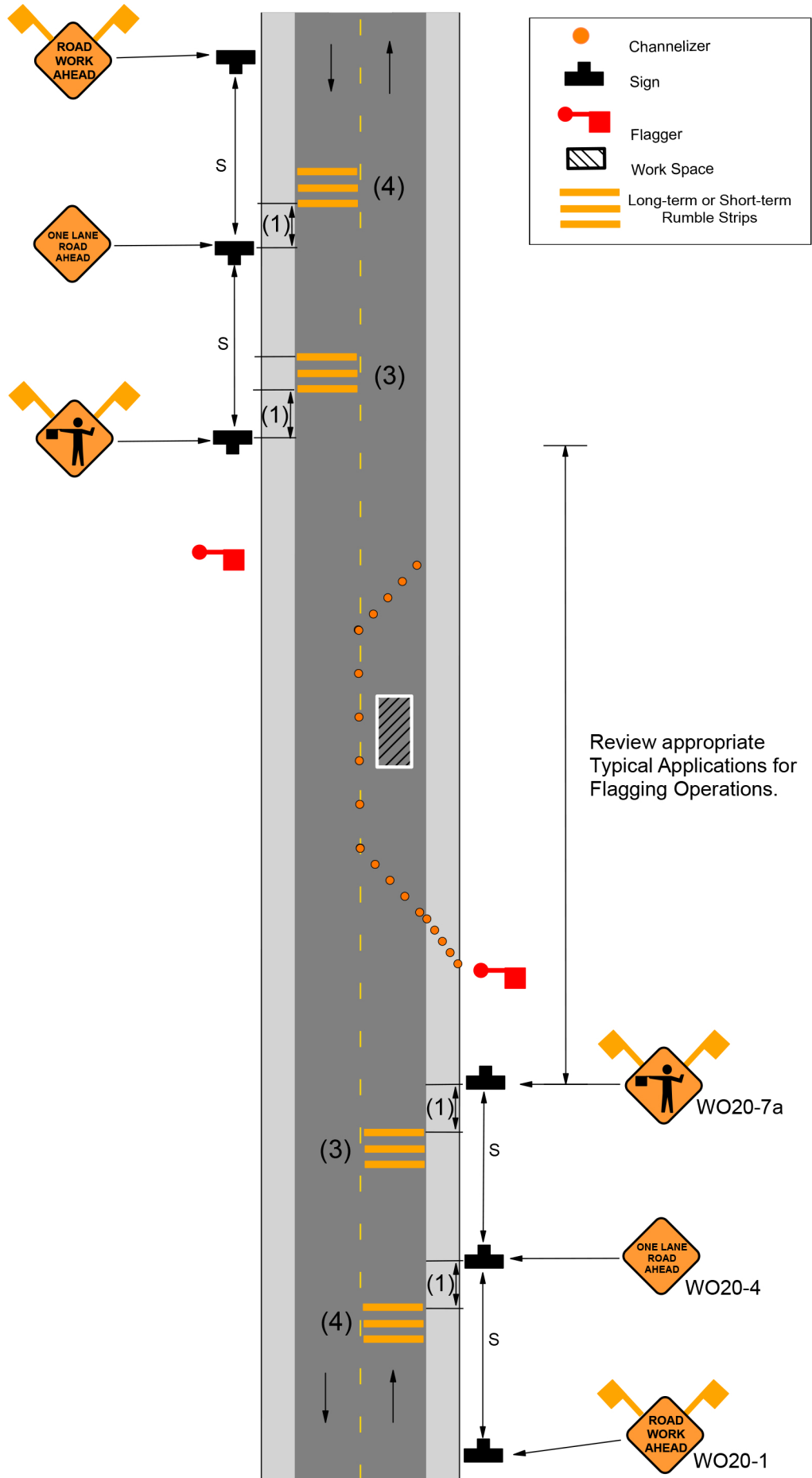
Figure: 616.6.87.1 Temporary Rumble Strip Placement in Flagging Operations
